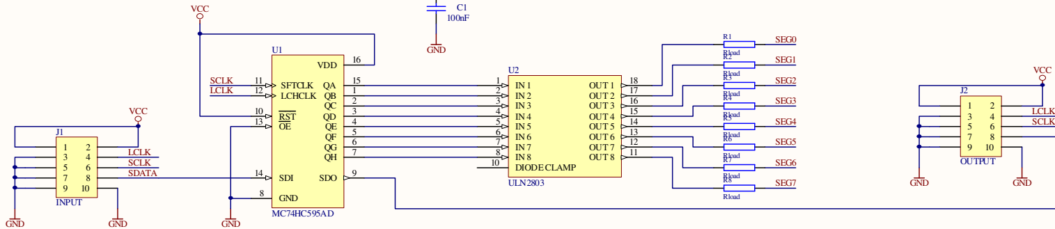
MCA2X 16 LED Controller
